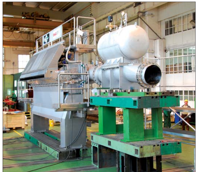
Intelli-Jet V™ headbox during pre-assembly at PMP
